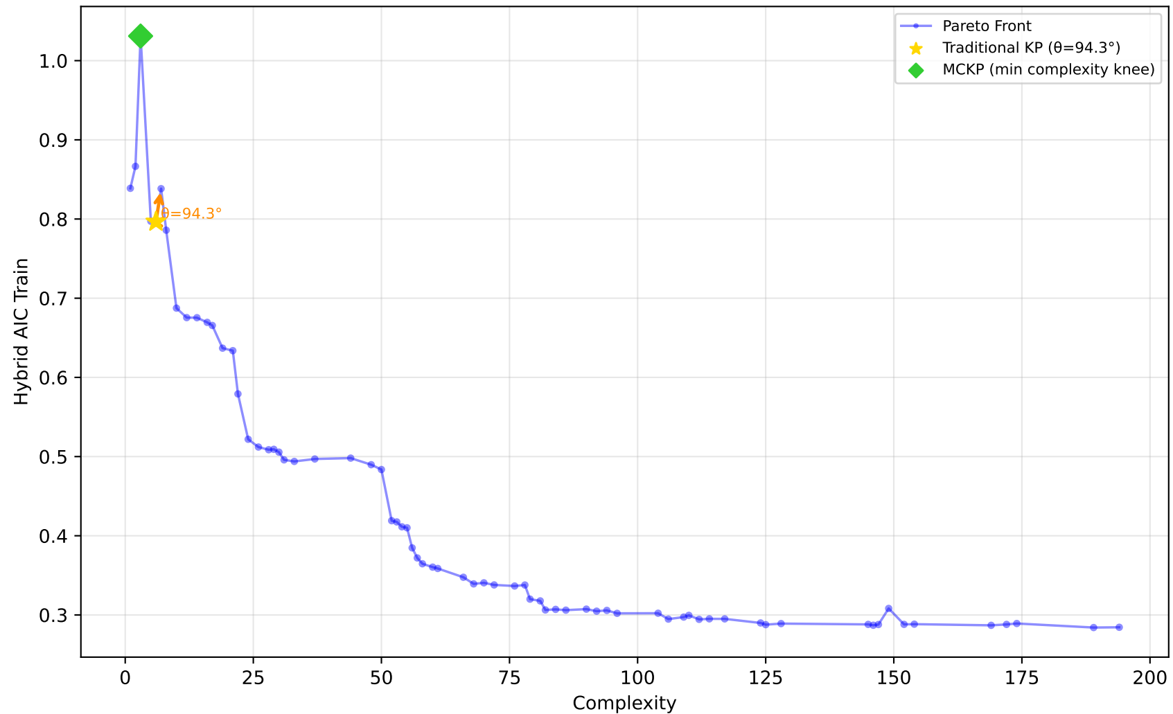
561_cpu - Run 25 - MVP - Hybrid AIC Train \lambda_1=0.50, \lambda_2=0.20, \lambda_3=0.00 | Difficulty: 1.00 | Method: hmr
