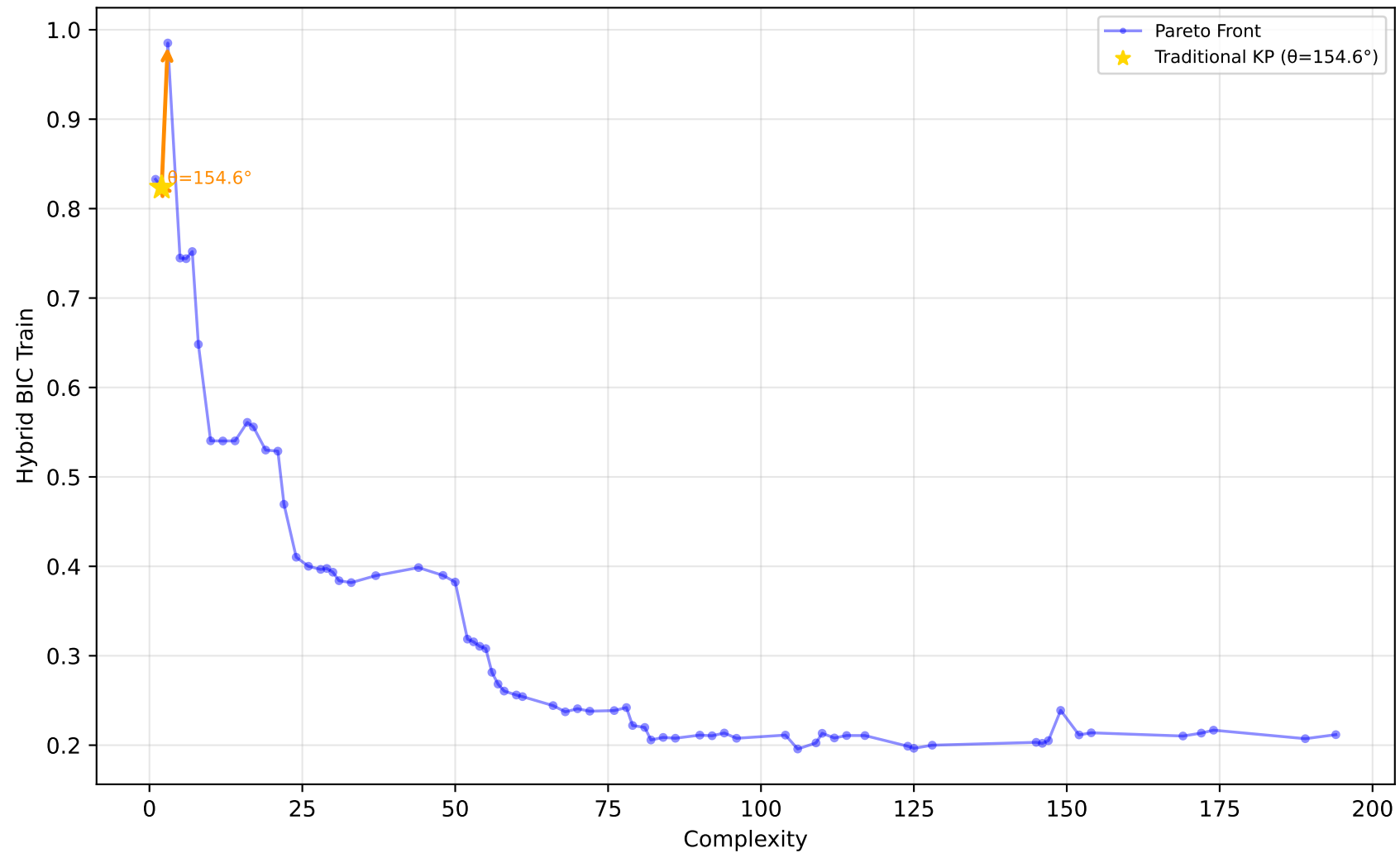
561_cpu - Run 25 - MVP - Hybrid BIC Train \lambda_1=0.70, \lambda_2=0.00, \lambda_3=0.10 | Difficulty: 1.00 | Method: hmr
