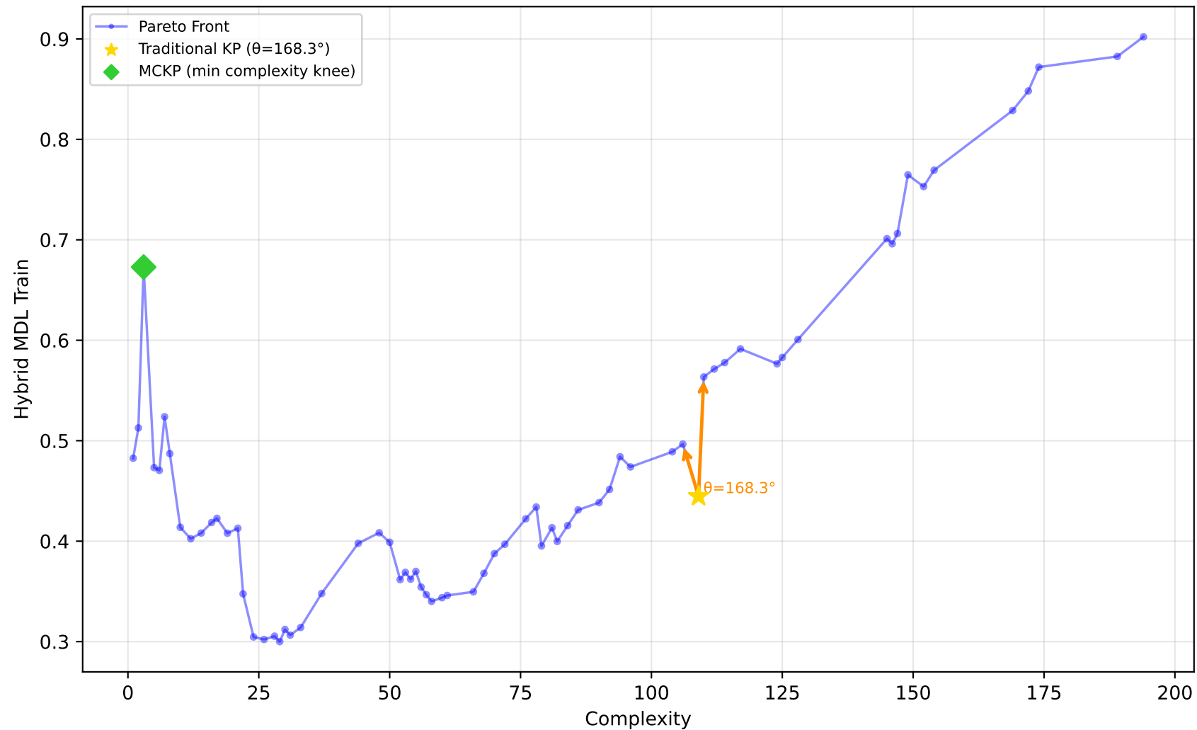
561_cpu - Run 25 - MVP - Hybrid MDL Train \lambda_1=0.50, \lambda_2=0.20, \lambda_3=0.00 | Difficulty: 1.00 | Method: hmr
