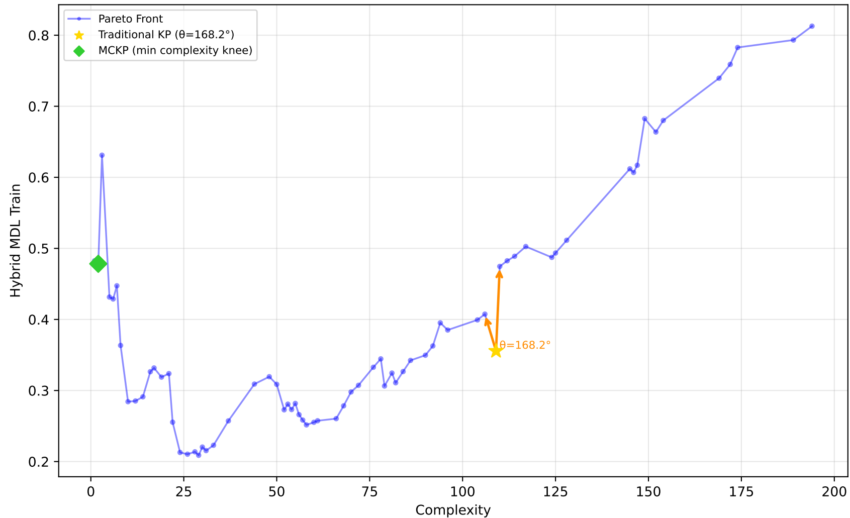
561_cpu - Run 25 - MVP - Hybrid MDL Train \lambda_1=0.70, \lambda_2=0.00, \lambda_3=0.10 | Difficulty: 1.00 | Method: hmr
