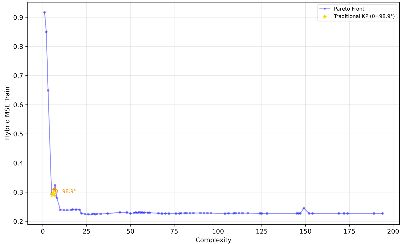
561_cpu - Run 25 - MVP - Hybrid MSE Train \lambda_1=0.50, \lambda_2=0.20, \lambda_3=0.00 | Difficulty: 1.00 | Method: hmr
