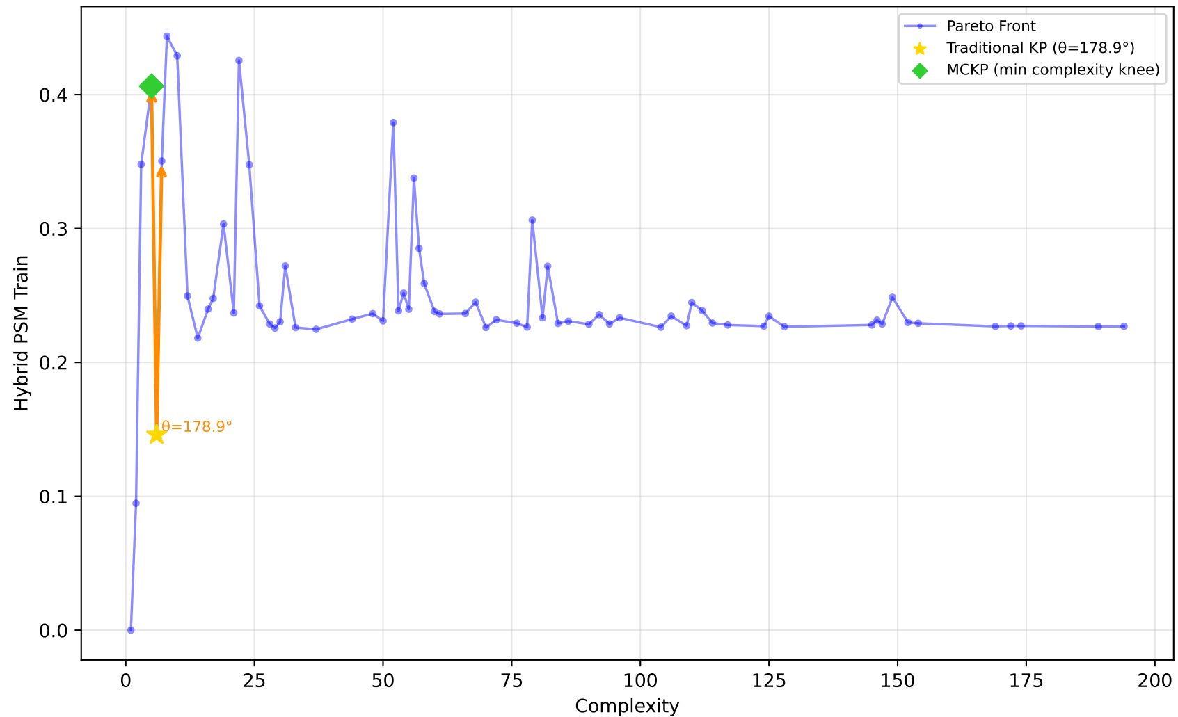
561_cpu - Run 25 - MVP - Hybrid PSM Train \lambda_1=0.50, \lambda_2=0.20, \lambda_3=0.00 | Difficulty: 1.00 | Method: hmr
