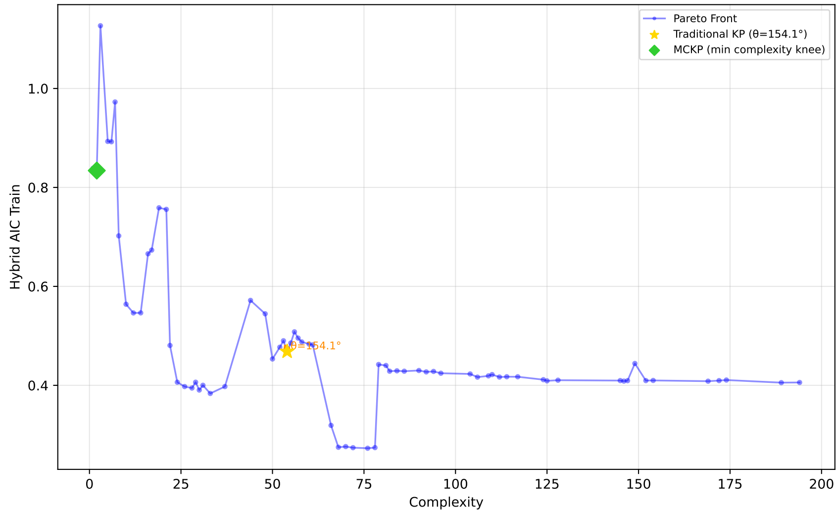
561_cpu - Run 25 - SVP - Hybrid AIC Train \lambda_1=0.90, \lambda_2=0.00, \lambda_3=0.30 | Difficulty: 1.00 | Method: hmr
