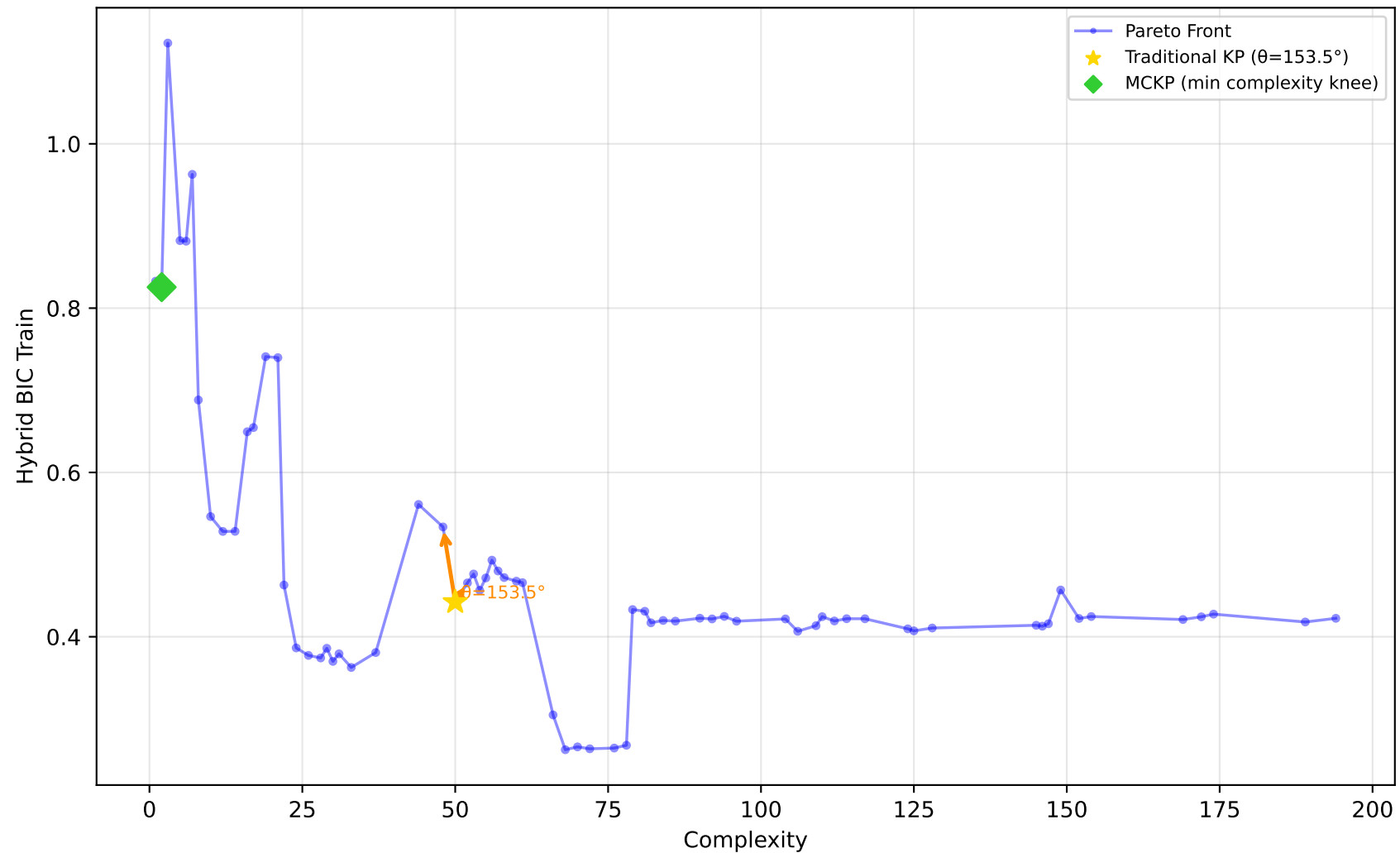
561_cpu - Run 25 - SVP - Hybrid BIC Train \lambda_1=0.90, \lambda_2=0.00, \lambda_3=0.30 | Difficulty: 1.00 | Method: hmr
