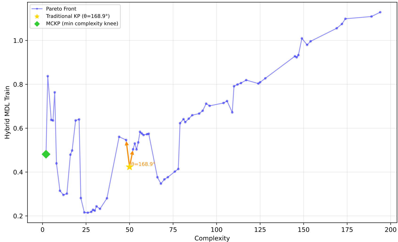
561_cpu - Run 25 - SVP - Hybrid MDL Train \lambda_1=1.00, \lambda_2=0.00, \lambda_3=0.40 | Difficulty: 1.00 | Method: hmr
