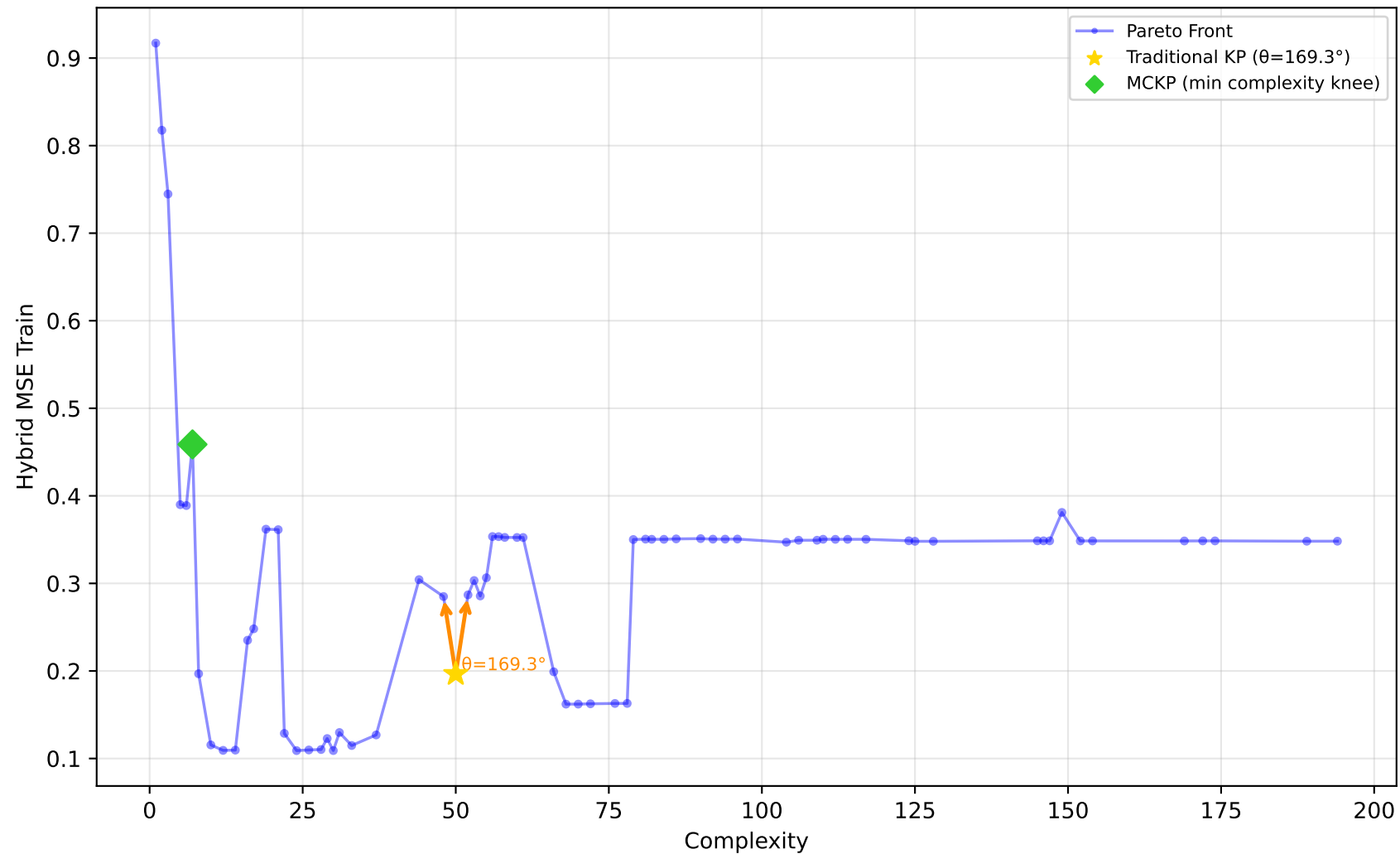
561_cpu - Run 25 - SVP - Hybrid MSE Train \lambda_1=0.90, \lambda_2=0.00, \lambda_3=0.30 | Difficulty: 1.00 | Method: hmr
