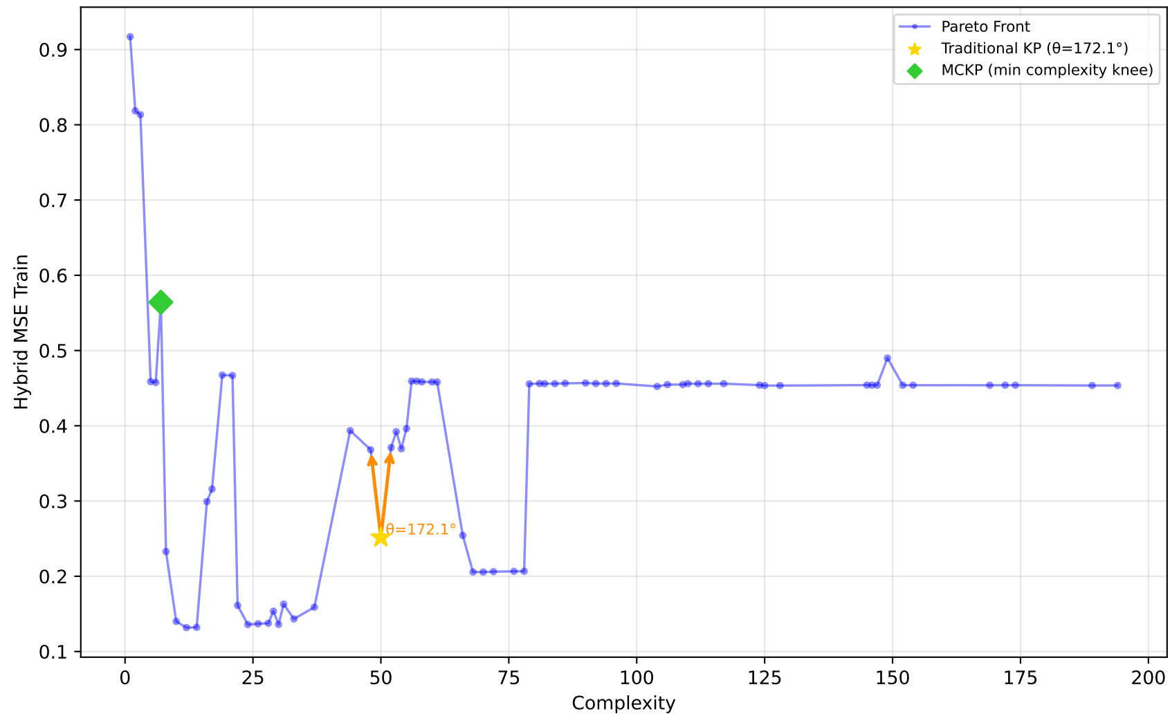
561_cpu - Run 25 - SVP - Hybrid MSE Train \lambda_1=1.00, \lambda_2=0.00, \lambda_3=0.40 | Difficulty: 1.00 | Method: hmr
