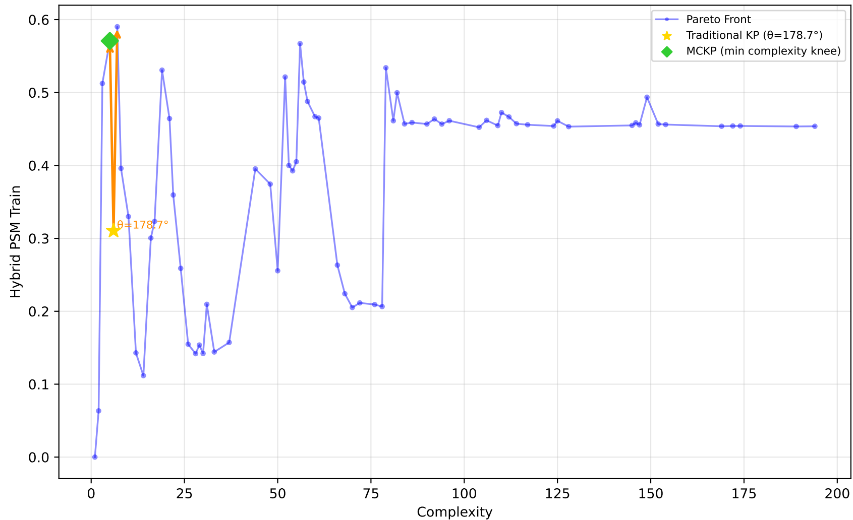
561_cpu - Run 25 - SVP - Hybrid PSM Train \lambda_1=1.00, \lambda_2=0.00, \lambda_3=0.40 | Difficulty: 1.00 | Method: hmr
