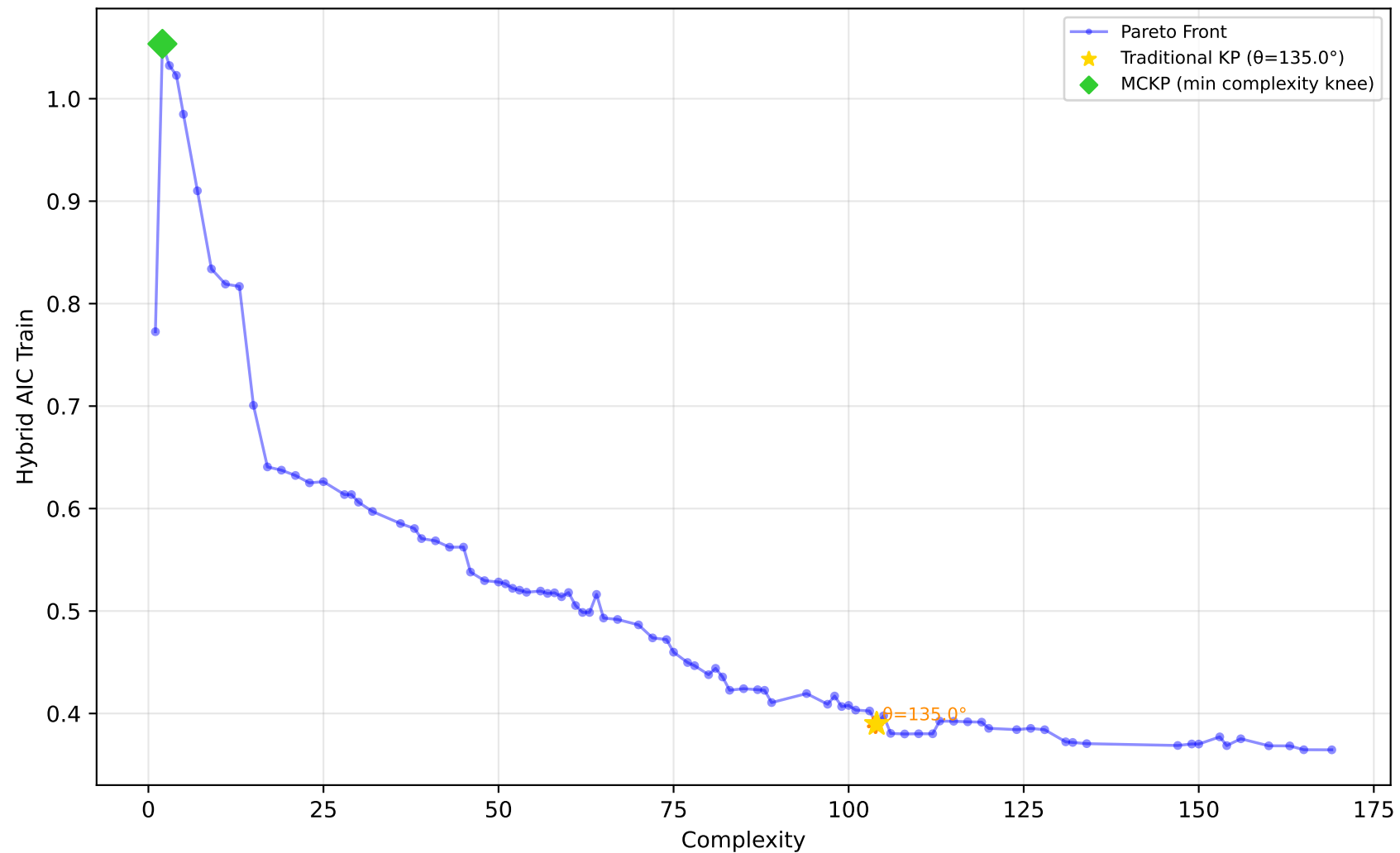
561_cpu - Run 26 - MVP - Hybrid AIC Train \lambda_1=0.50, \lambda_2=0.20, \lambda_3=0.00 | Difficulty: 0.41 | Method: mckp
