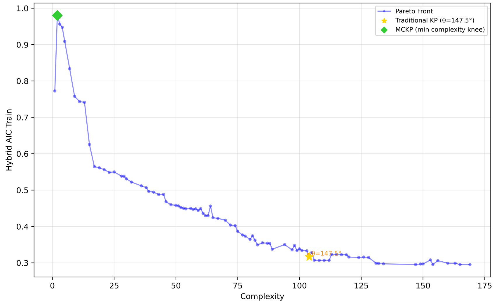
561_cpu - Run 26 - MVP - Hybrid AIC Train \lambda_1=0.70, \lambda_2=0.00, \lambda_3=0.10 | Difficulty: 0.41 | Method: mckp
