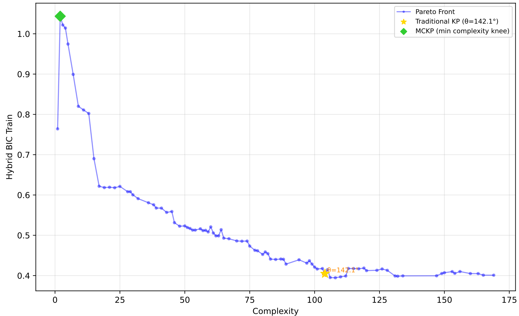
561_cpu - Run 26 - MVP - Hybrid BIC Train \lambda_1=0.50, \lambda_2=0.20, \lambda_3=0.00 | Difficulty: 0.41 | Method: mckp
