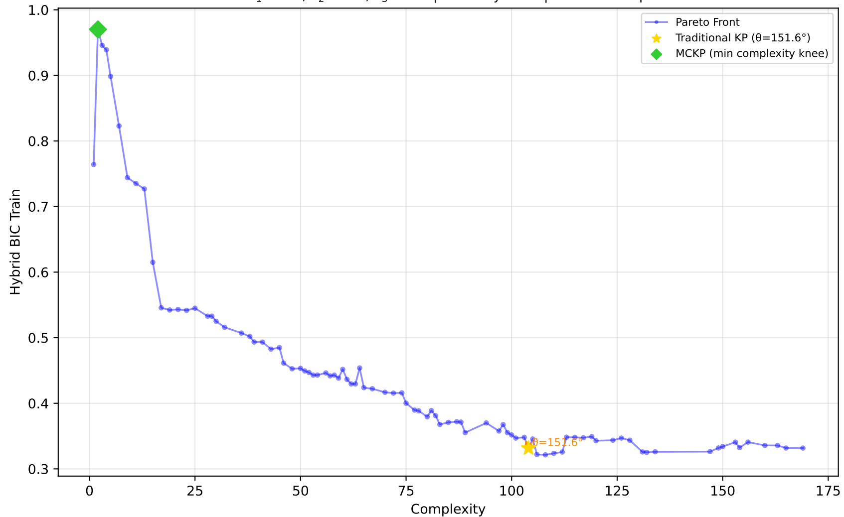
561_cpu - Run 26 - MVP - Hybrid BIC Train \lambda_1=0.70, \lambda_2=0.00, \lambda_3=0.10 | Difficulty: 0.41 | Method: mckp
