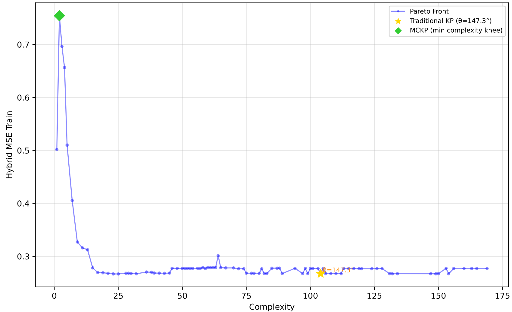
561_cpu - Run 26 - MVP - Hybrid MSE Train \lambda_1=0.50, \lambda_2=0.20, \lambda_3=0.00 | Difficulty: 0.41 | Method: mckp
