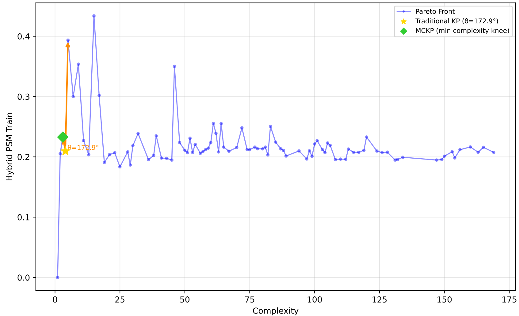
561_cpu - Run 26 - MVP - Hybrid PSM Train \lambda_1=0.70, \lambda_2=0.00, \lambda_3=0.10 | Difficulty: 0.41 | Method: mckp
