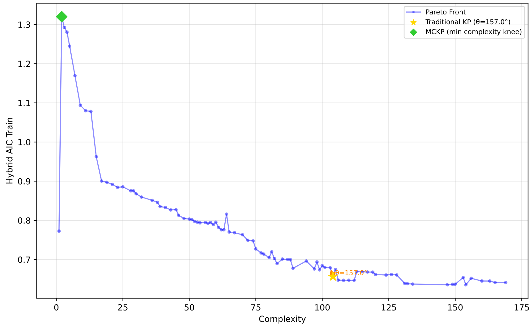
561_cpu - Run 26 - SVP - Hybrid AIC Train \lambda_1=1.00, \lambda_2=0.00, \lambda_3=0.40 | Difficulty: 0.41 | Method: mckp
