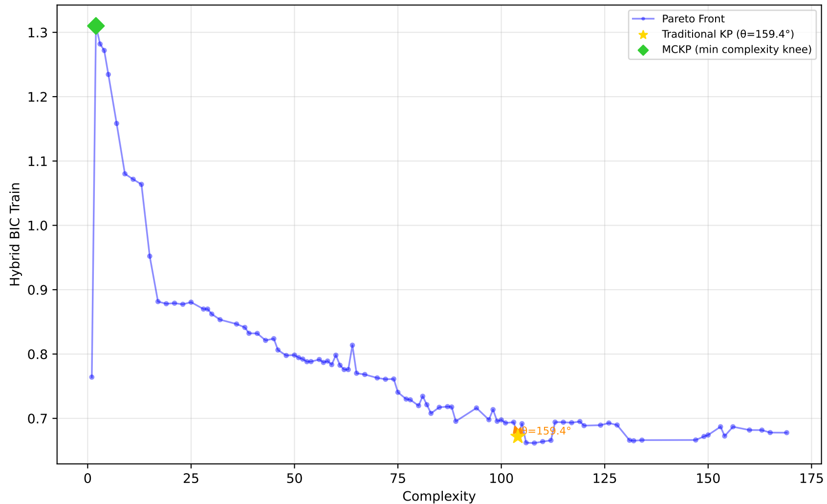
561_cpu - Run 26 - SVP - Hybrid BIC Train \lambda_1=1.00 , \lambda_2=0.00 , \lambda_3=0.40 | Difficulty: 0.41 | Method: mckp
