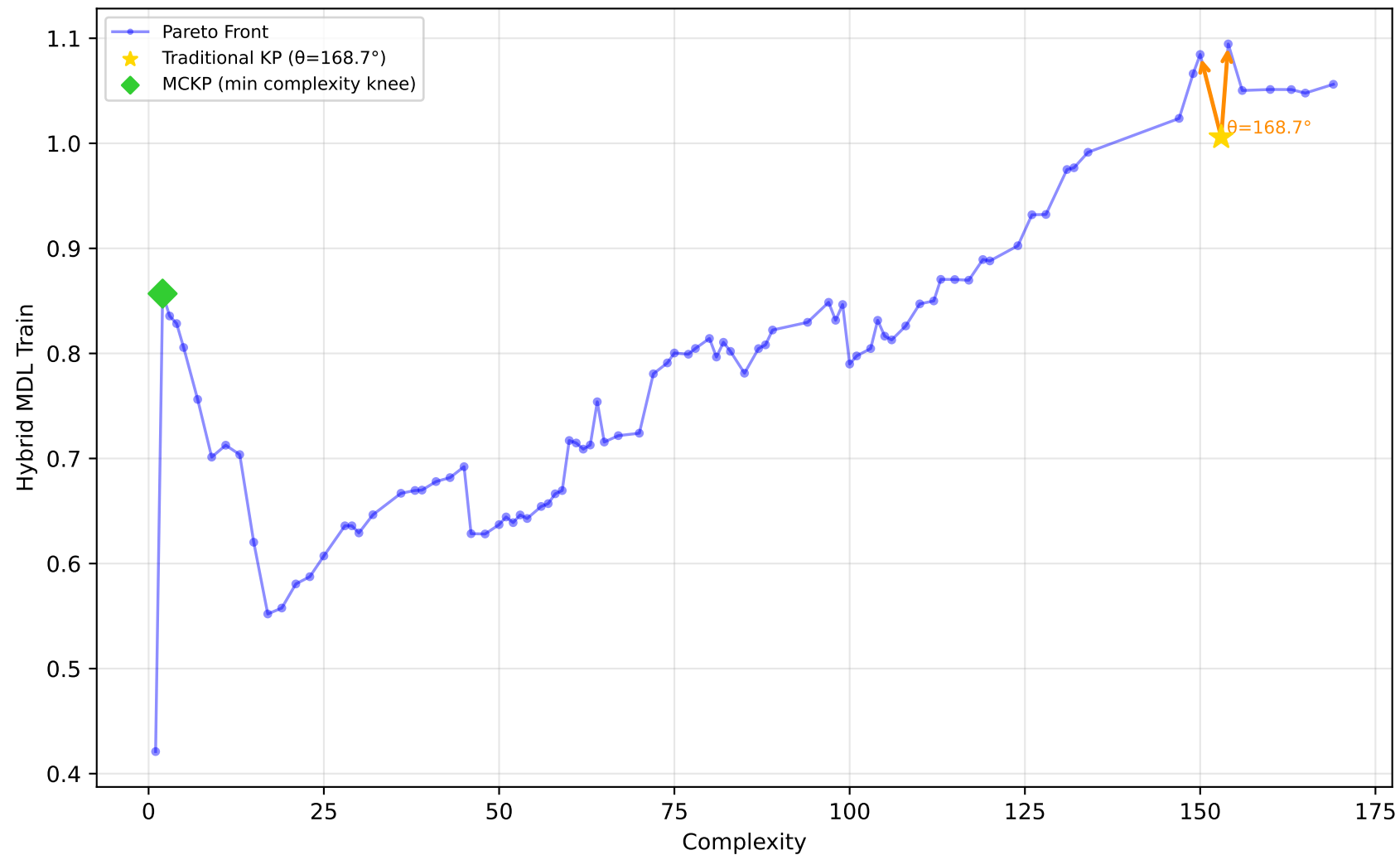
561_cpu - Run 26 - SVP - Hybrid MDL Train \lambda_1=0.90, \lambda_2=0.00, \lambda_3=0.30 | Difficulty: 0.41 | Method: mckp
