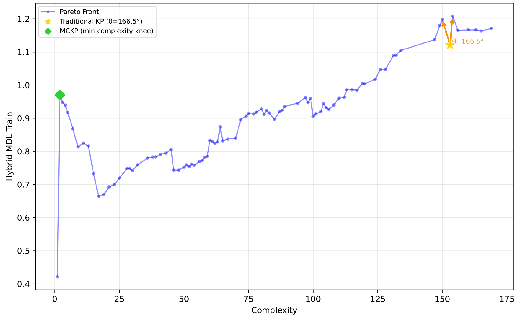
561_cpu - Run 26 - SVP - Hybrid MDL Train \lambda_1=1.00, \lambda_2=0.00, \lambda_3=0.40 | Difficulty: 0.41 | Method: mckp
