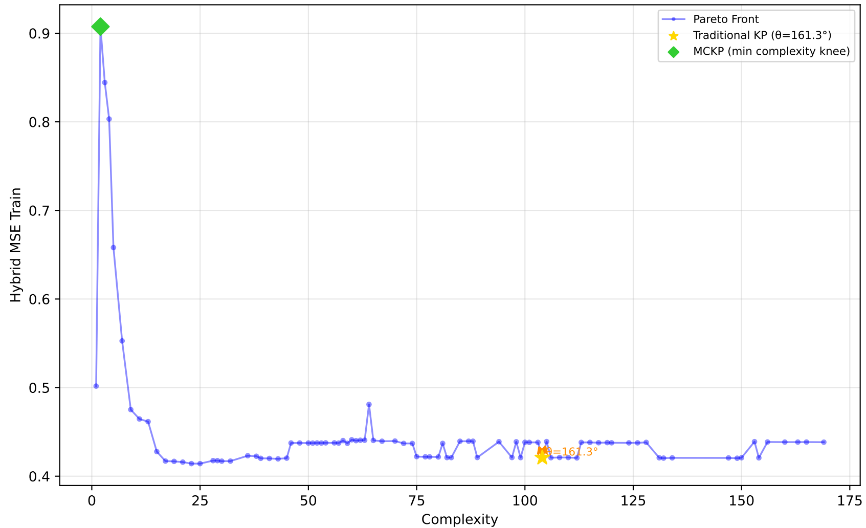
561_cpu - Run 26 - SVP - Hybrid MSE Train \lambda_1=0.90, \lambda_2=0.00, \lambda_3=0.30 | Difficulty: 0.41 | Method: mckp
