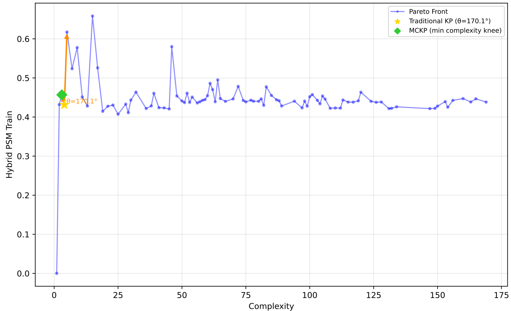
561_cpu - Run 26 - SVP - Hybrid PSM Train \lambda_1=0.90, \lambda_2=0.00, \lambda_3=0.30 | Difficulty: 0.41 | Method: mckp
