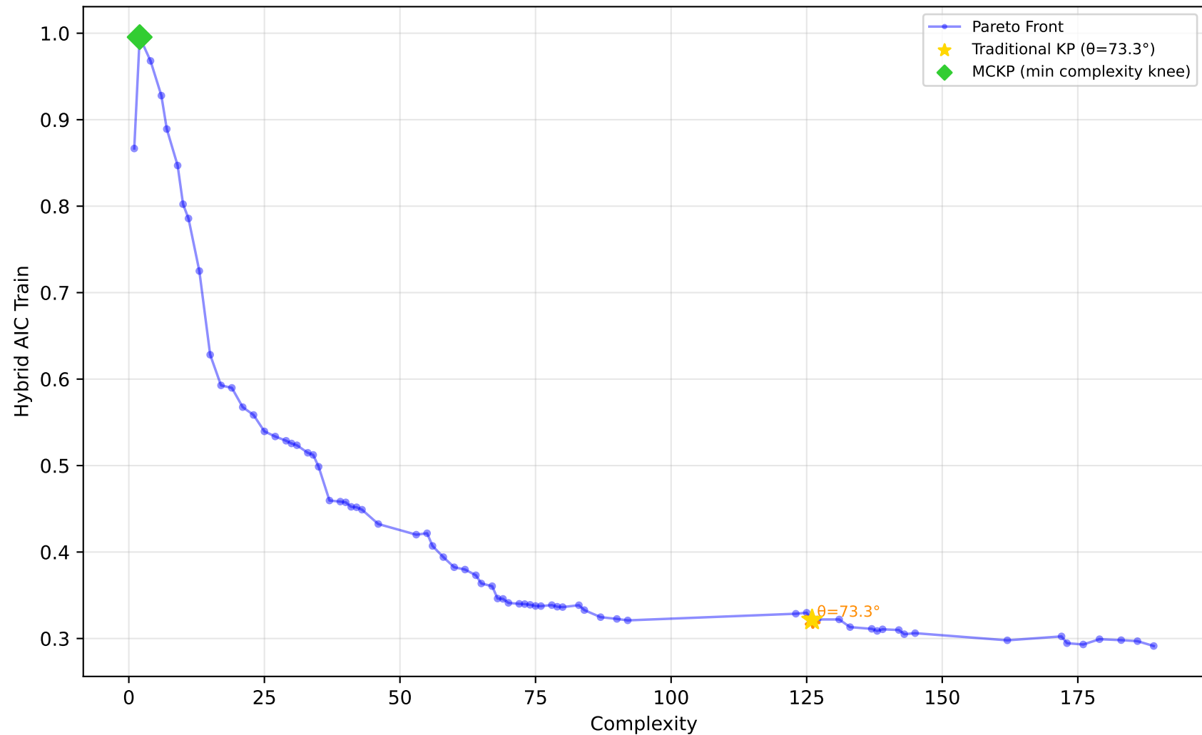
561_cpu - Run 27 - MVP - Hybrid AIC Train \lambda_1=0.50, \lambda_2=0.20, \lambda_3=0.00 | Difficulty: 1.00 | Method: hmr
