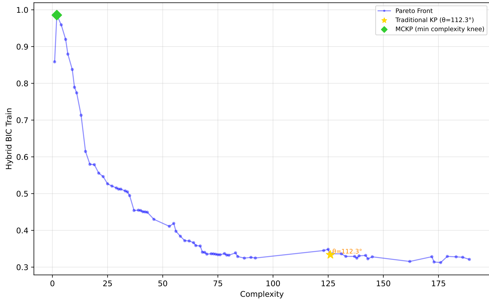
561_cpu - Run 27 - MVP - Hybrid BIC Train \lambda_1=0.50, \lambda_2=0.20, \lambda_3=0.00 | Difficulty: 1.00 | Method: hmr
