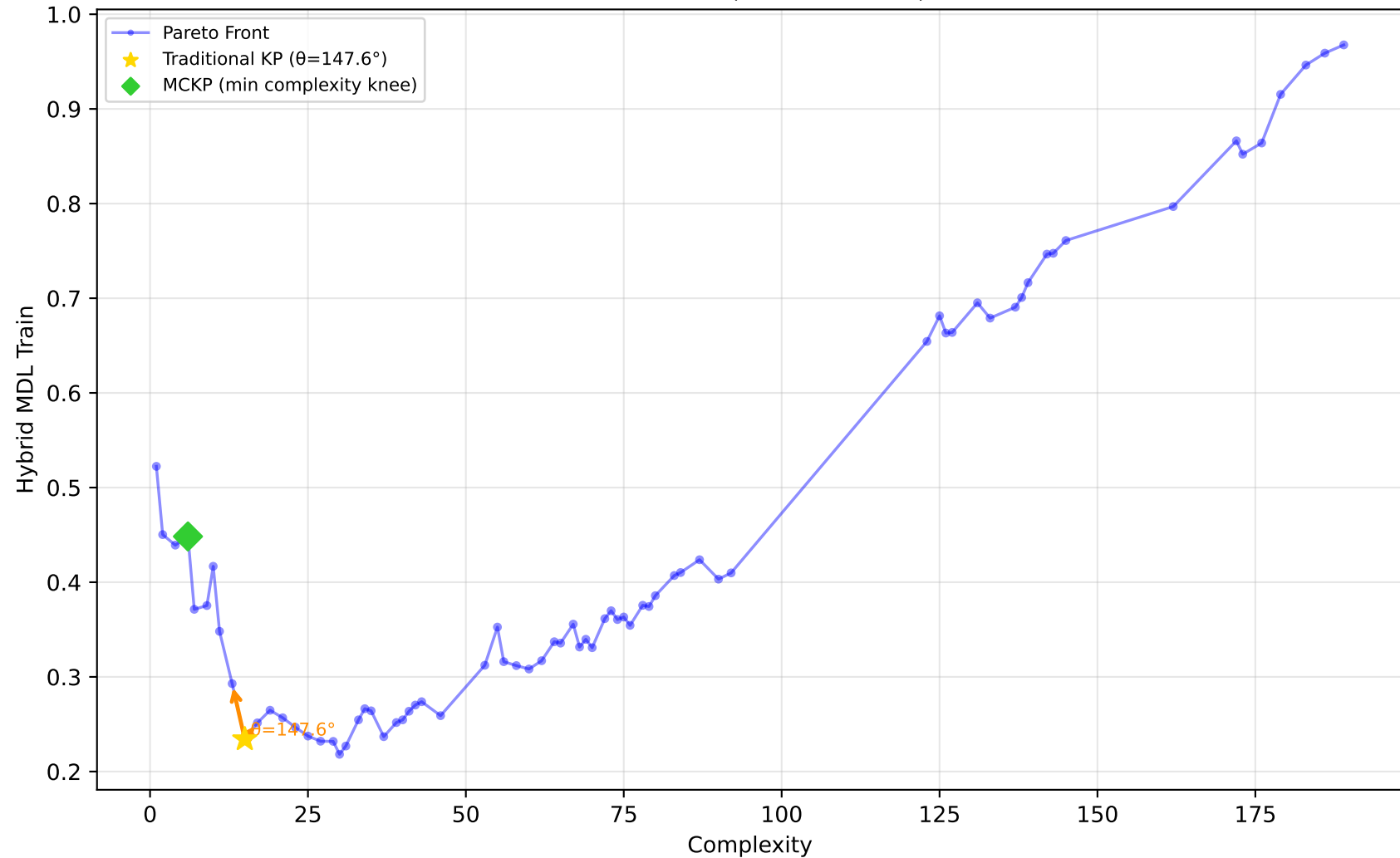
561_cpu - Run 27 - MVP - Hybrid MDL Train \lambda_1=0.70, \lambda_2=0.00, \lambda_3=0.10 | Difficulty: 1.00 | Method: hmr
