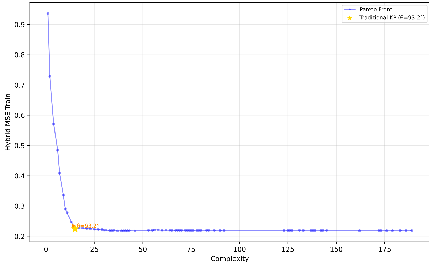
561_cpu - Run 27 - MVP - Hybrid MSE Train \lambda_1=0.50, \lambda_2=0.20, \lambda_3=0.00 | Difficulty: 1.00 | Method: hmr
