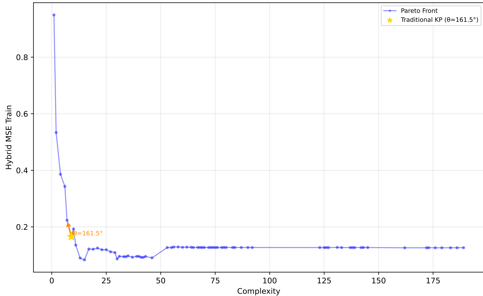
561_cpu - Run 27 - MVP - Hybrid MSE Train \lambda_1=0.70, \lambda_2=0.00, \lambda_3=0.10 | Difficulty: 1.00 | Method: hmr
