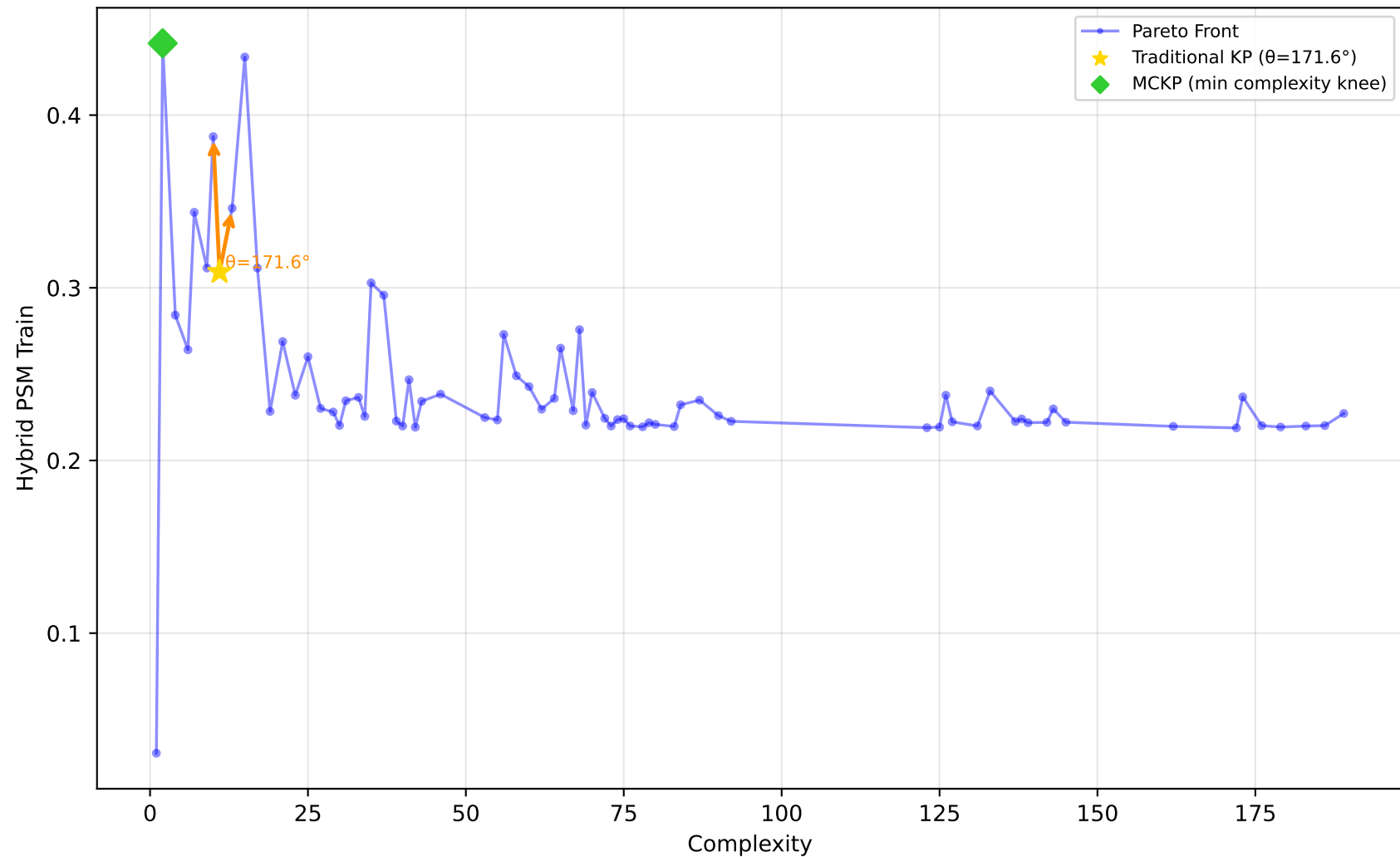
561_cpu - Run 27 - MVP - Hybrid PSM Train \lambda_1=0.50, \lambda_2=0.20, \lambda_3=0.00 | Difficulty: 1.00 | Method: hmr
