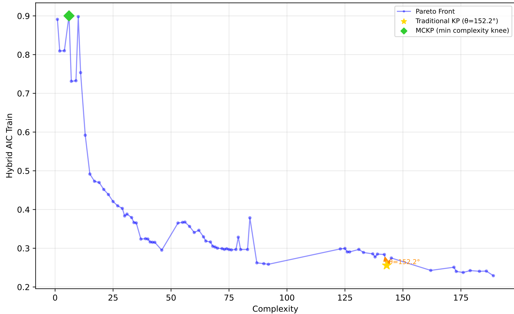
561_cpu - Run 27 - SVP - Hybrid AIC Train \lambda_1=0.90, \lambda_2=0.00, \lambda_3=0.30 | Difficulty: 1.00 | Method: hmr
