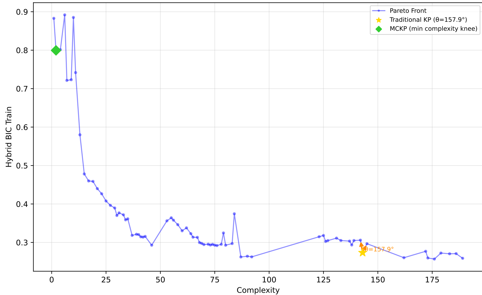
561_cpu - Run 27 - SVP - Hybrid BIC Train \lambda_1=0.90, \lambda_2=0.00, \lambda_3=0.30 | Difficulty: 1.00 | Method: hmr
