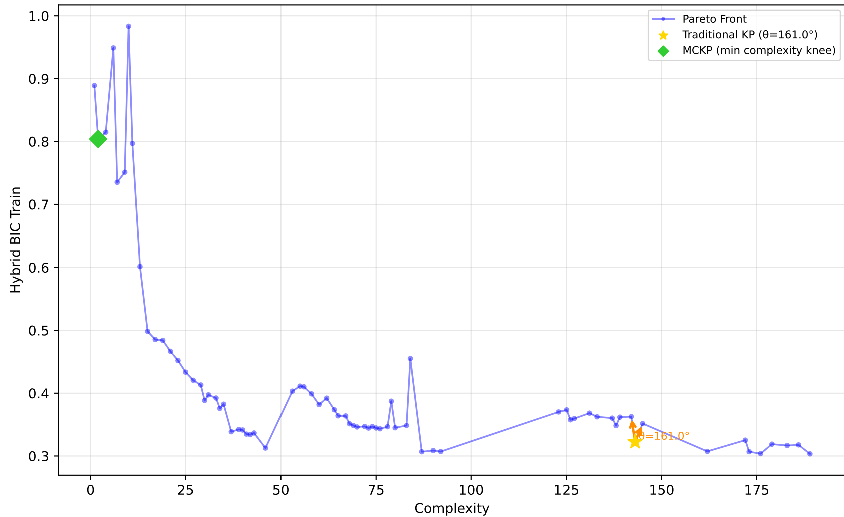
561_cpu - Run 27 - SVP - Hybrid BIC Train \lambda_1=1.00, \lambda_2=0.00, \lambda_3=0.40 | Difficulty: 1.00 | Method: hmr
