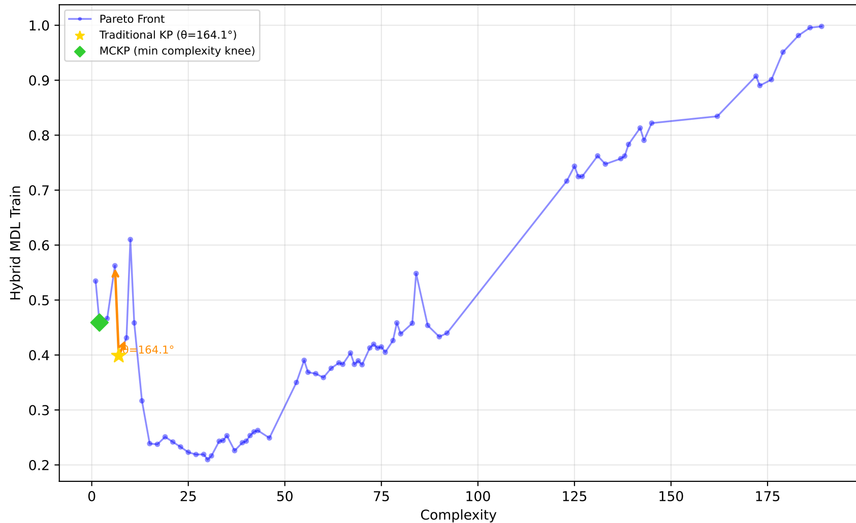
561_cpu - Run 27 - SVP - Hybrid MDL Train \lambda_1=0.90, \lambda_2=0.00, \lambda_3=0.30 | Difficulty: 1.00 | Method: hmr
