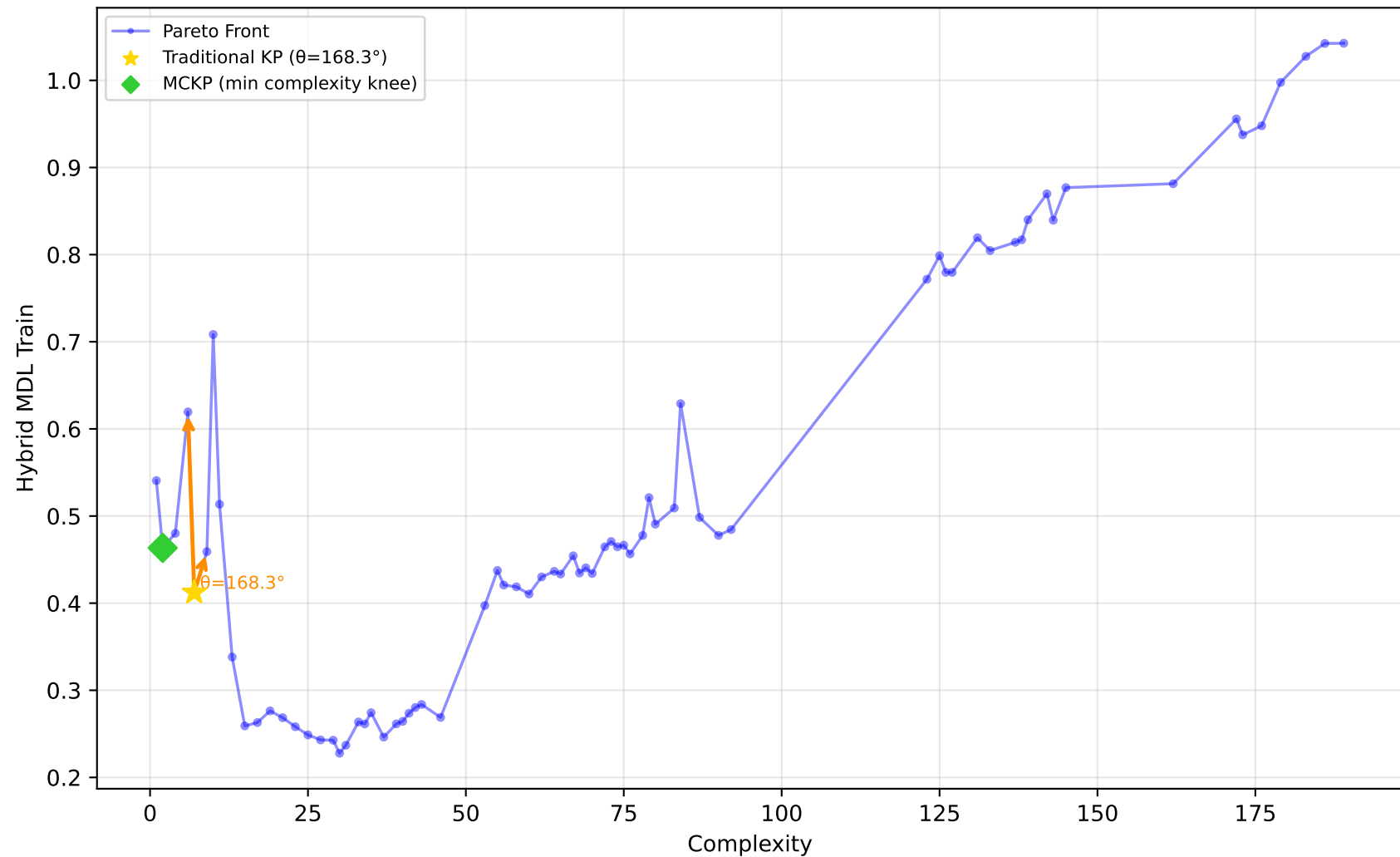
561_cpu - Run 27 - SVP - Hybrid MDL Train \lambda_1=1.00, \lambda_2=0.00, \lambda_3=0.40 | Difficulty: 1.00 | Method: hmr
