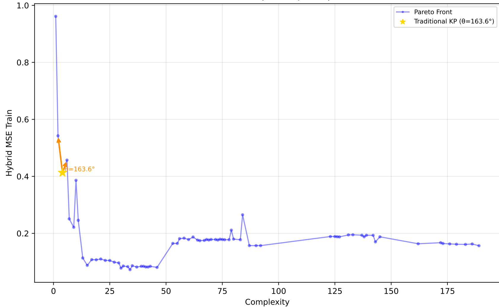
561_cpu - Run 27 - SVP - Hybrid MSE Train \lambda_1=0.90, \lambda_2=0.00, \lambda_3=0.30 | Difficulty: 1.00 | Method: hmr
