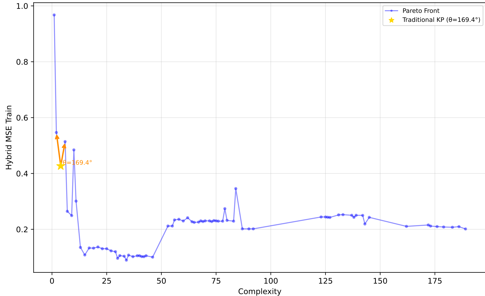
561_cpu - Run 27 - SVP - Hybrid MSE Train \lambda_1=1.00, \lambda_2=0.00, \lambda_3=0.40 | Difficulty: 1.00 | Method: hmr
