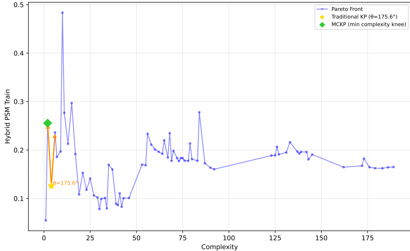
561_cpu - Run 27 - SVP - Hybrid PSM Train \lambda_1=0.90, \lambda_2=0.00, \lambda_3=0.30 | Difficulty: 1.00 | Method: hmr
