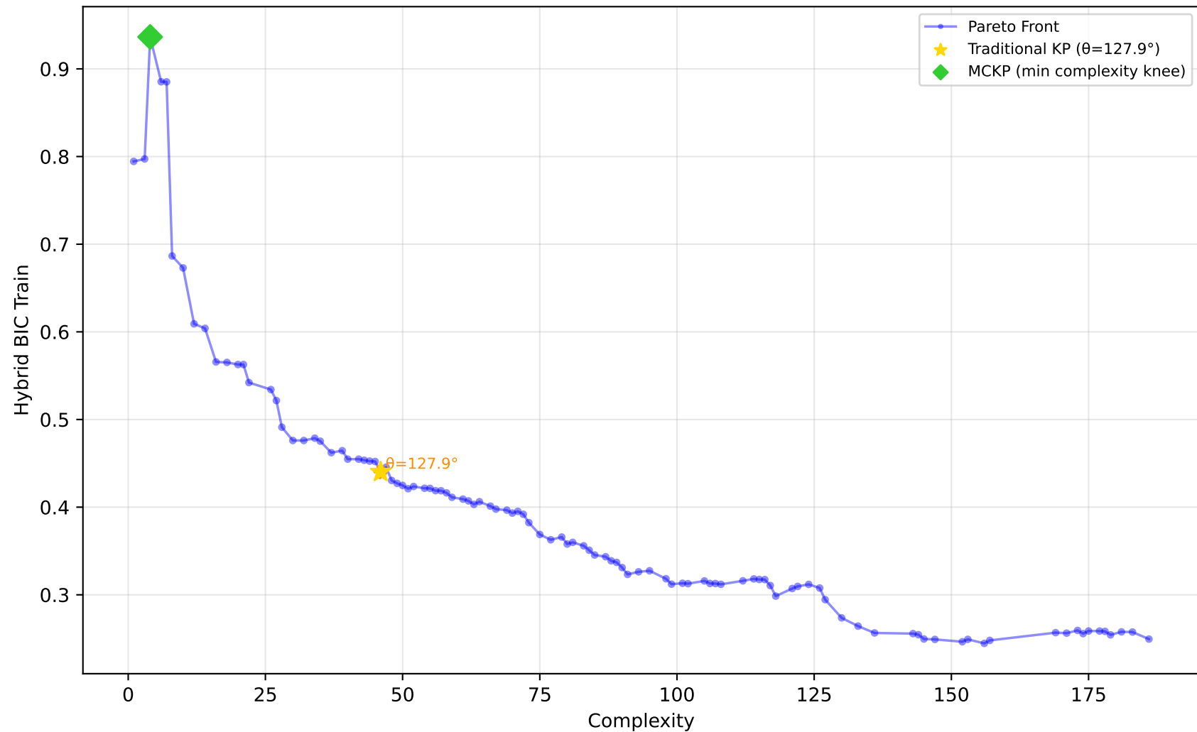
561_cpu - Run 28 - MVP - Hybrid BIC Train \lambda_1=0.50, \lambda_2=0.20, \lambda_3=0.00 | Difficulty: 1.00 | Method: hmr
