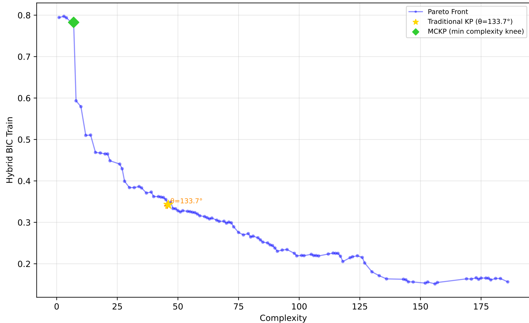
561_cpu - Run 28 - MVP - Hybrid BIC Train \lambda_1=0.70, \lambda_2=0.00, \lambda_3=0.10 | Difficulty: 1.00 | Method: hmr
