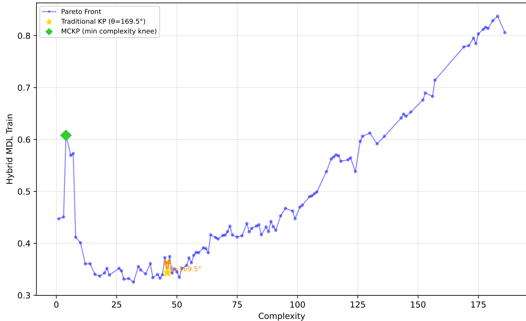
561_cpu - Run 28 - MVP - Hybrid MDL Train \lambda_1=0.50, \lambda_2=0.20, \lambda_3=0.00 | Difficulty: 1.00 | Method: hmr
