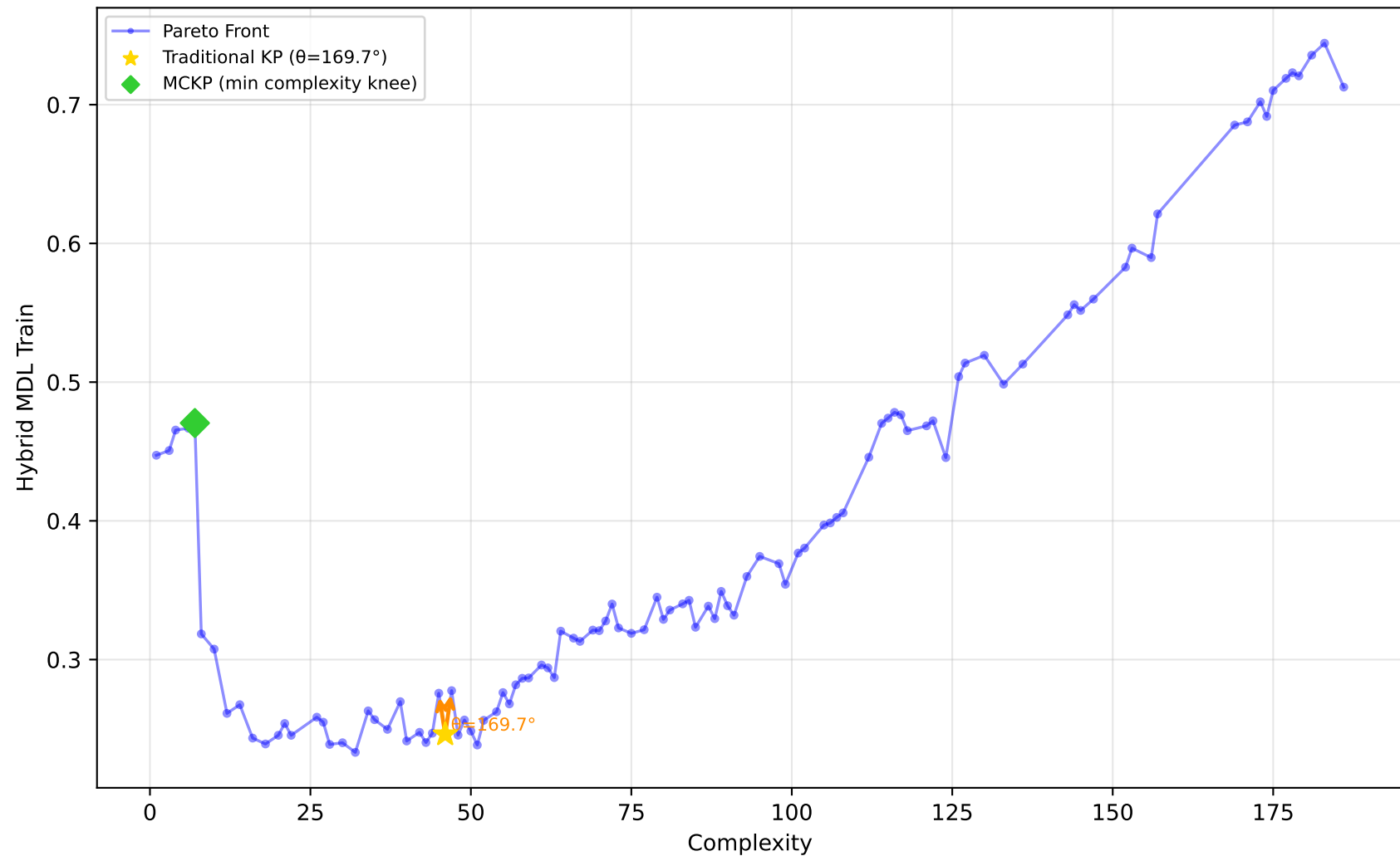
561_cpu - Run 28 - MVP - Hybrid MDL Train \lambda_1=0.70, \lambda_2=0.00, \lambda_3=0.10 | Difficulty: 1.00 | Method: hmr
