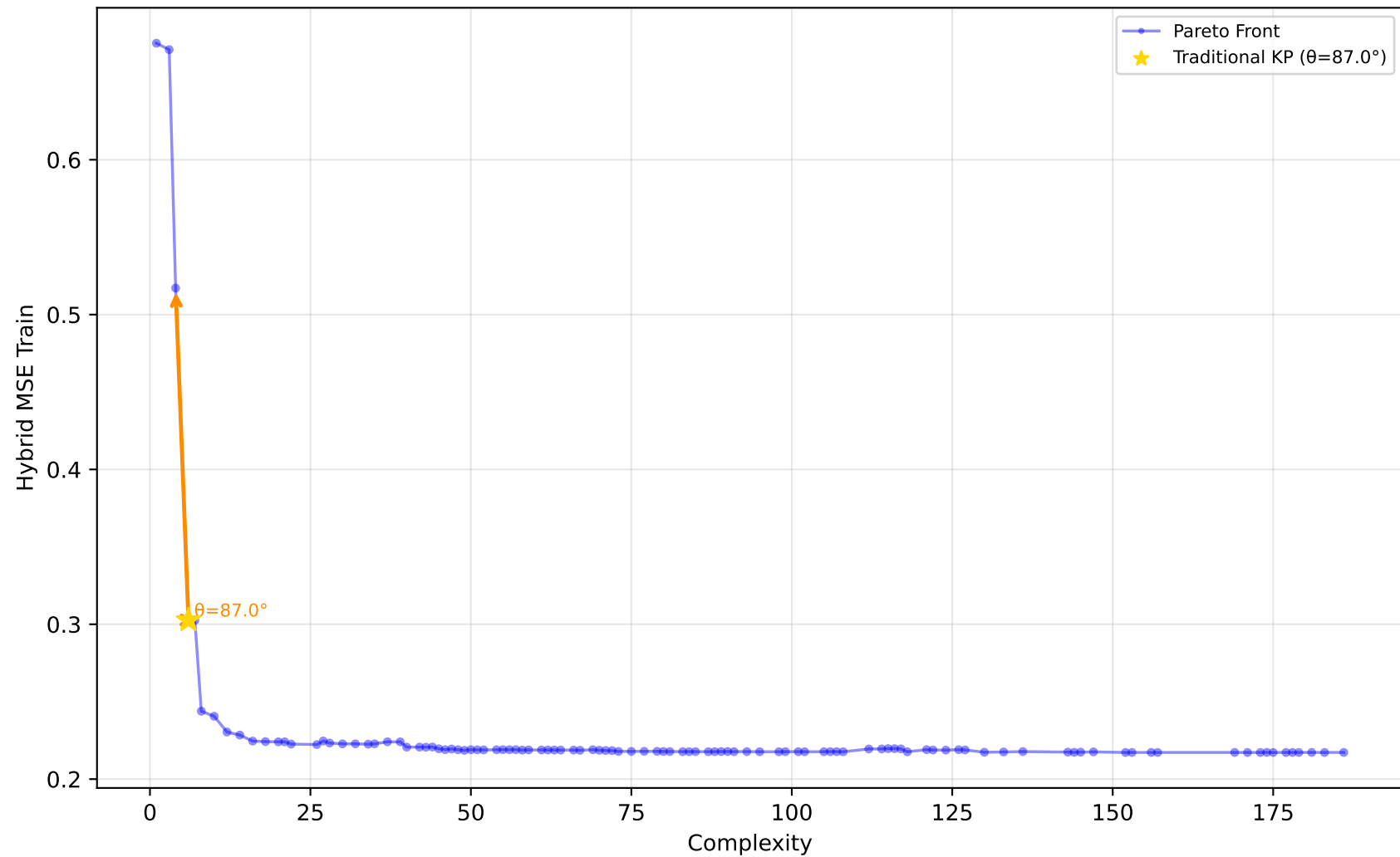
561_cpu - Run 28 - MVP - Hybrid MSE Train \lambda_1=0.50, \lambda_2=0.20, \lambda_3=0.00 | Difficulty: 1.00 | Method: hmr
