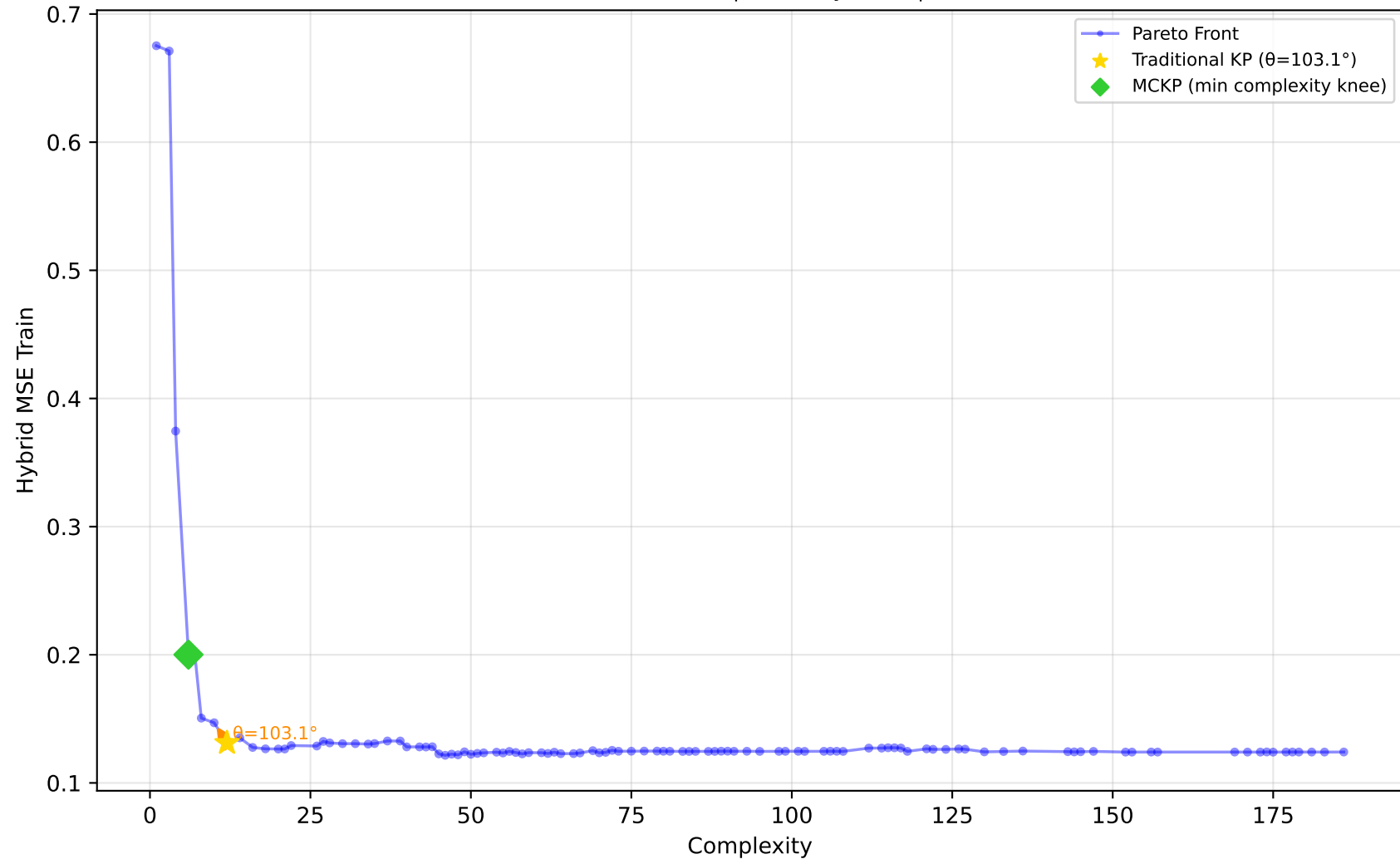
561_cpu - Run 28 - MVP - Hybrid MSE Train \lambda_1=0.70, \lambda_2=0.00, \lambda_3=0.10 | Difficulty: 1.00 | Method: hmr
