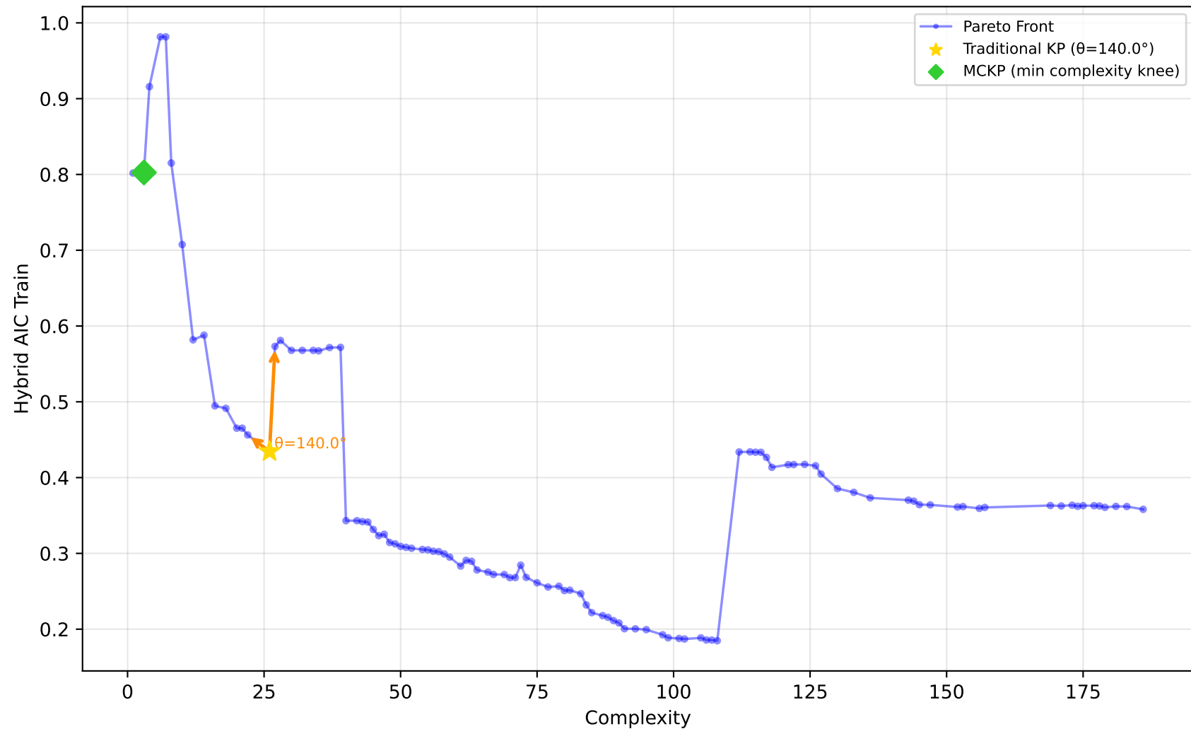
561_cpu - Run 28 - SVP - Hybrid AIC Train \lambda_1=0.90, \lambda_2=0.00, \lambda_3=0.30 | Difficulty: 1.00 | Method: hmr
