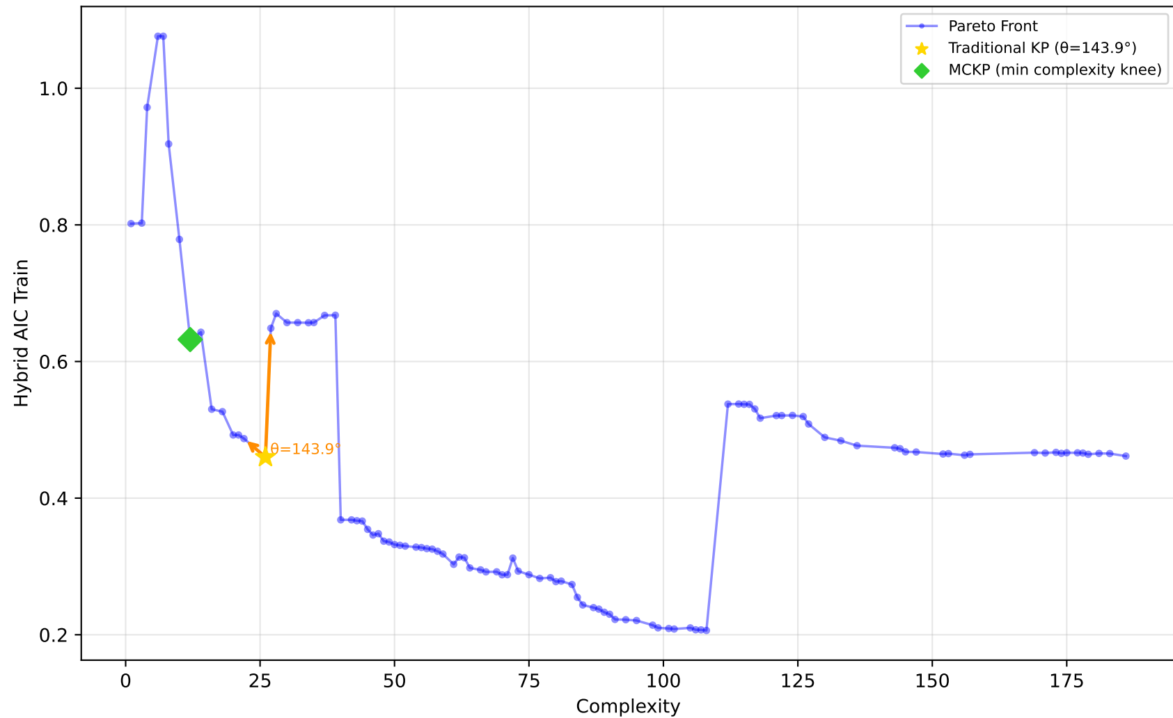
561_cpu - Run 28 - SVP - Hybrid AIC Train \lambda_1=1.00, \lambda_2=0.00, \lambda_3=0.40 | Difficulty: 1.00 | Method: hmr
