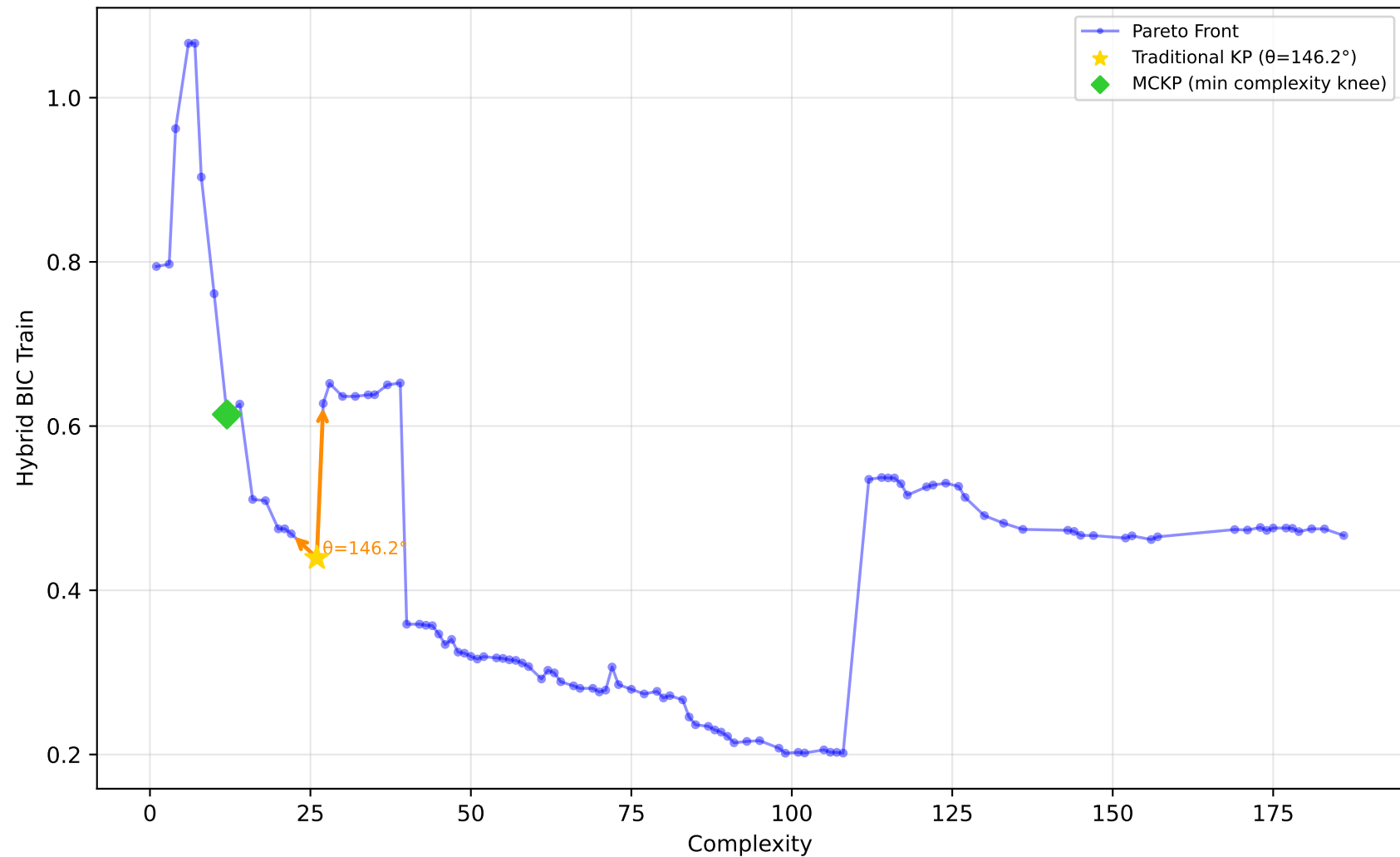
561_cpu - Run 28 - SVP - Hybrid BIC Train \lambda_1=1.00, \lambda_2=0.00, \lambda_3=0.40 | Difficulty: 1.00 | Method: hmr
