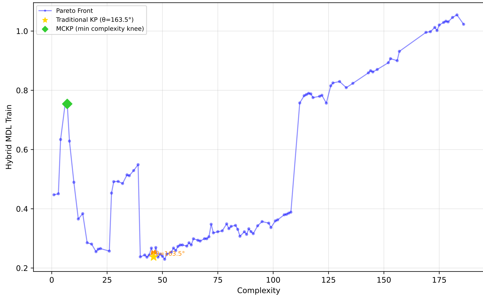
561_cpu - Run 28 - SVP - Hybrid MDL Train \lambda_1=1.00, \lambda_2=0.00, \lambda_3=0.40 | Difficulty: 1.00 | Method: hmr
