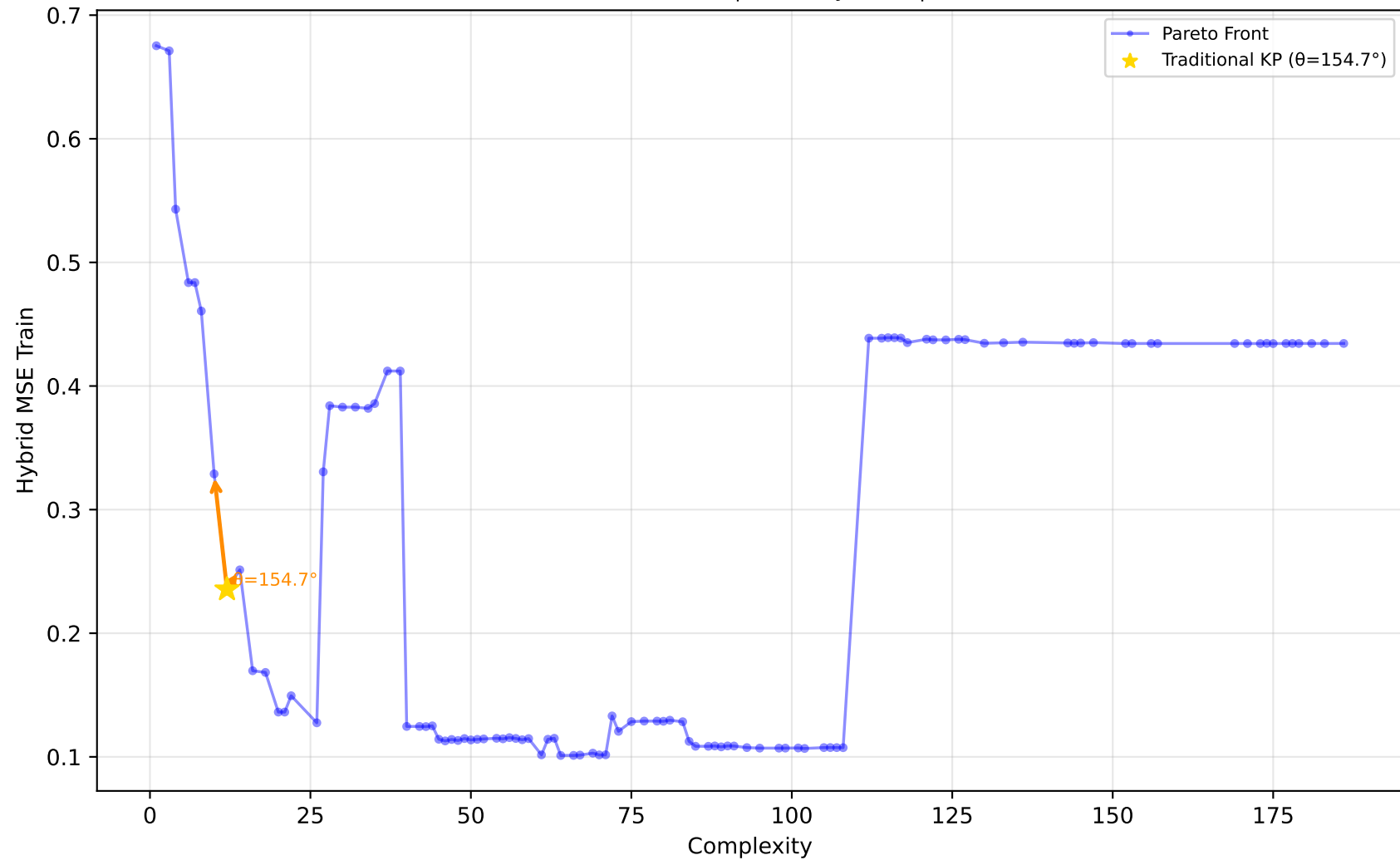
561_cpu - Run 28 - SVP - Hybrid MSE Train \lambda_1=1.00, \lambda_2=0.00, \lambda_3=0.40 | Difficulty: 1.00 | Method: hmr
