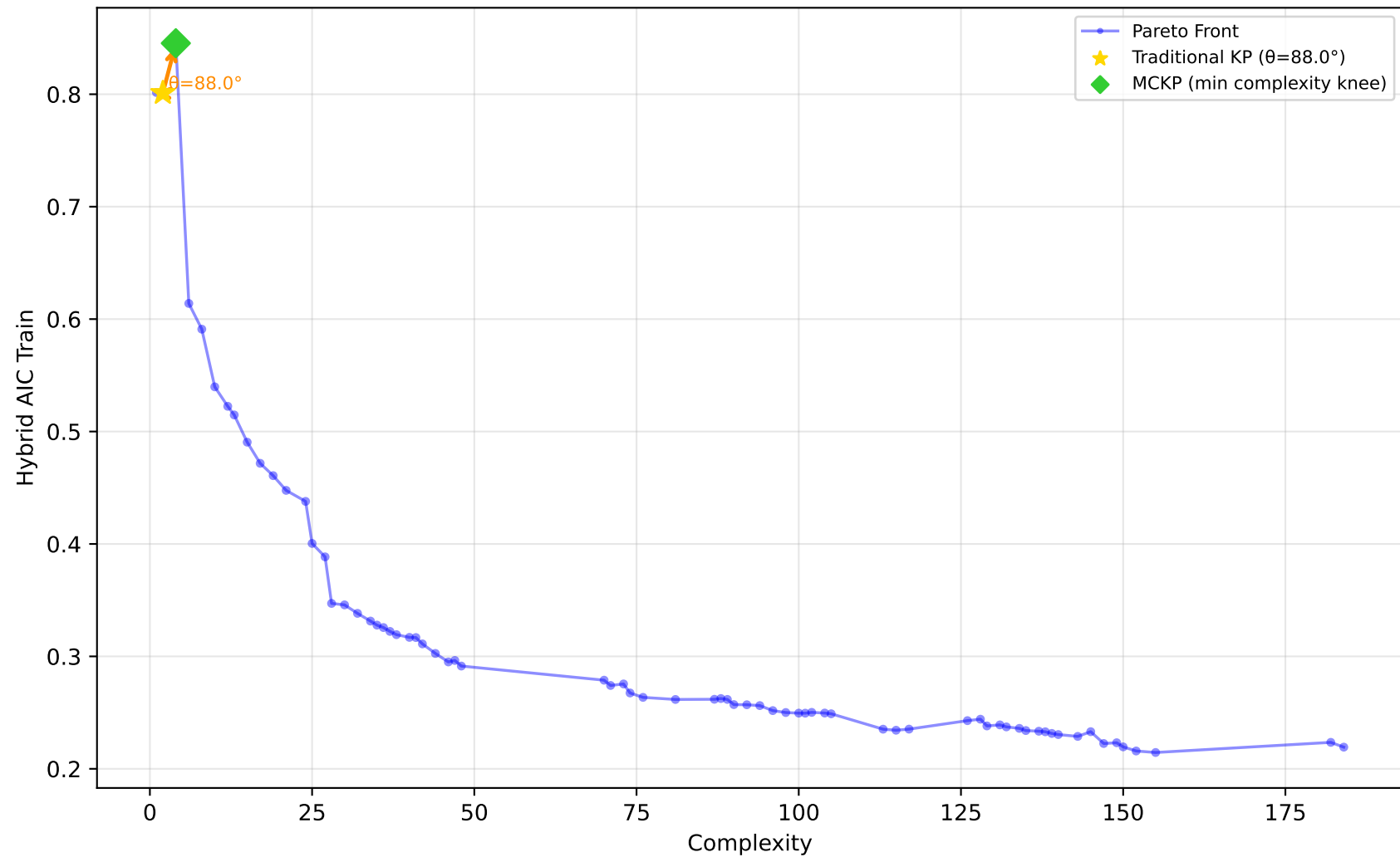
561_cpu - Run 29 - MVP - Hybrid AIC Train \lambda_1=0.70, \lambda_2=0.00, \lambda_3=0.10 | Difficulty: 1.00 | Method: hmr
